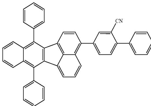
compound 1
