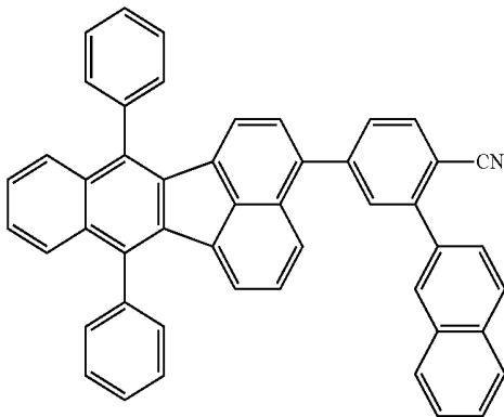
compound 23
