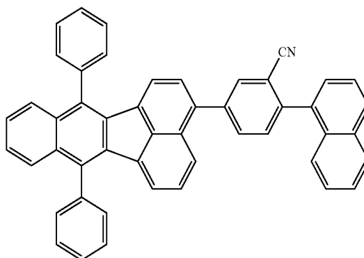
compound 2
