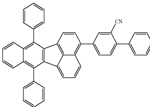
compound 2
