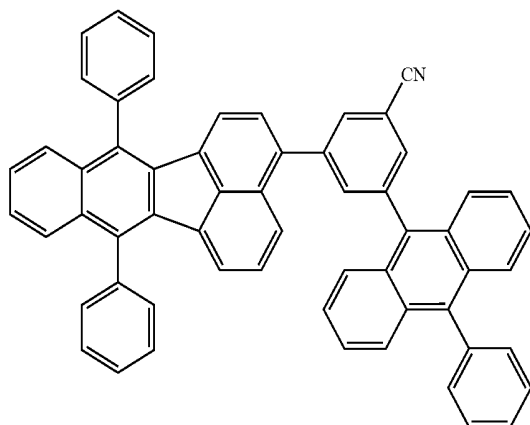
compound 9
