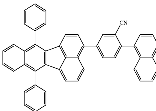
compound 3
