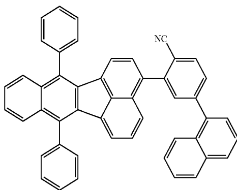
compound 18
