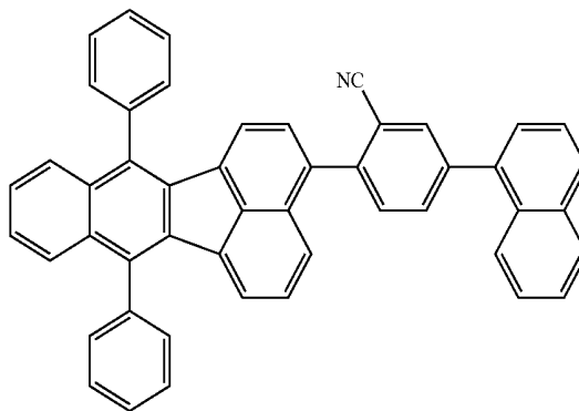
compound 12
