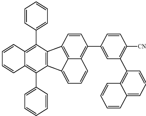
compound 22
