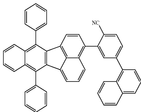
compound 17
