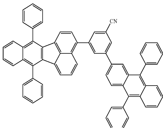
compound 10
