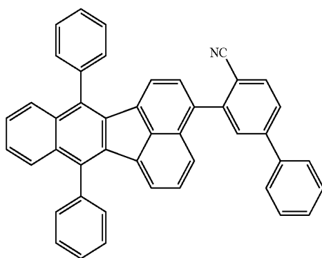
compound 16
