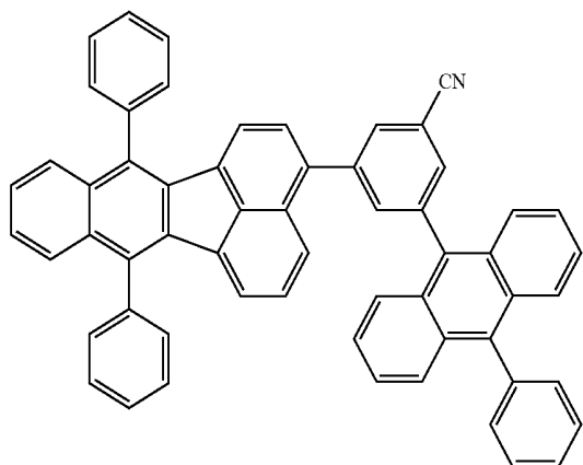
compound 10
