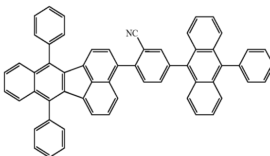
compound 14
