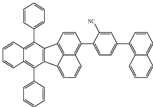
compound 12
