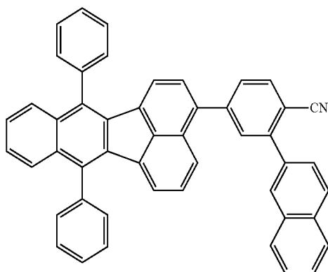
compound 23
