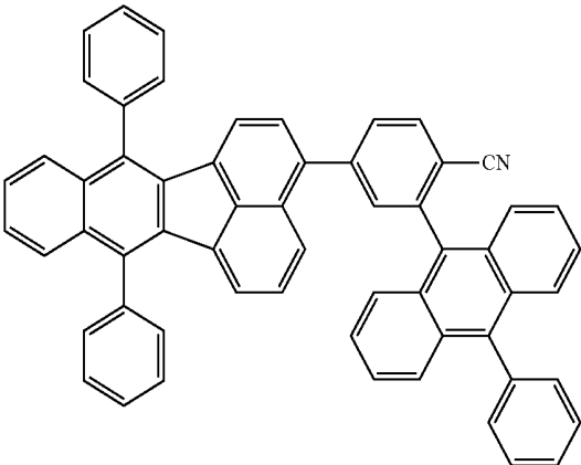
compound 25
