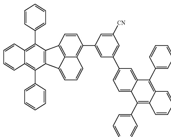
compound 11
