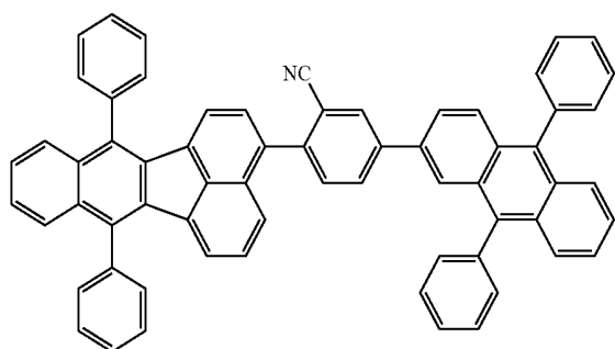
compound 15
