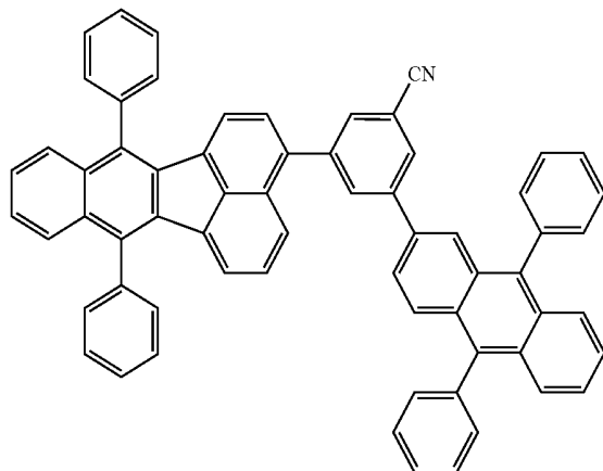
compound 10
