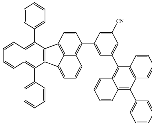
compound 10
