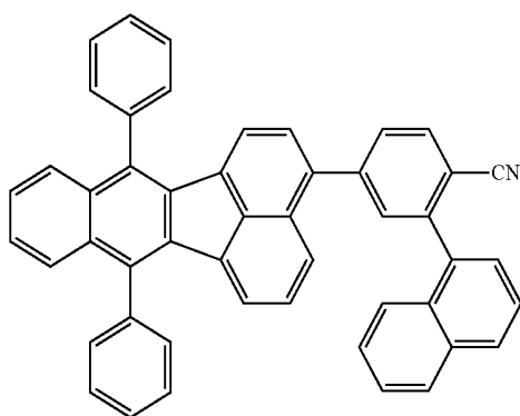
compound 23
