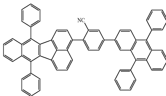
compound 15
