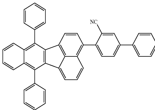
compound 11
