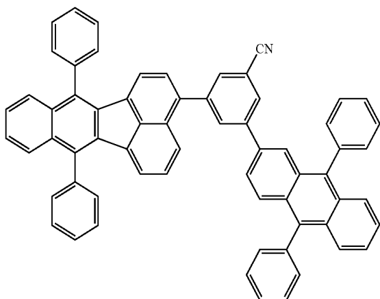
compound 11
