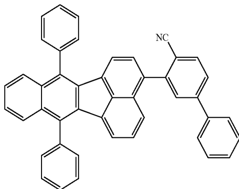
compound 16
