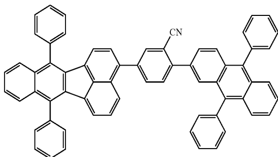
compound 5
