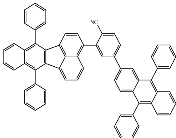
compound 21
