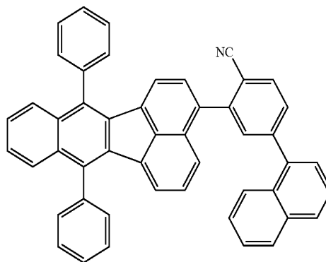
compound 17
