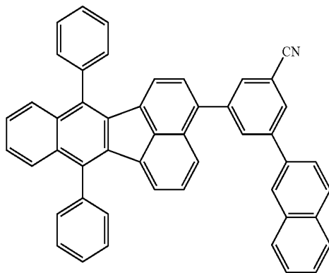
compound 8
