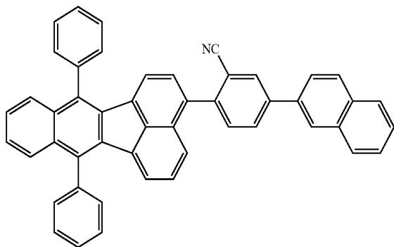
compound 13
