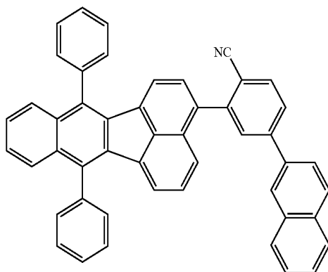
compound 18
