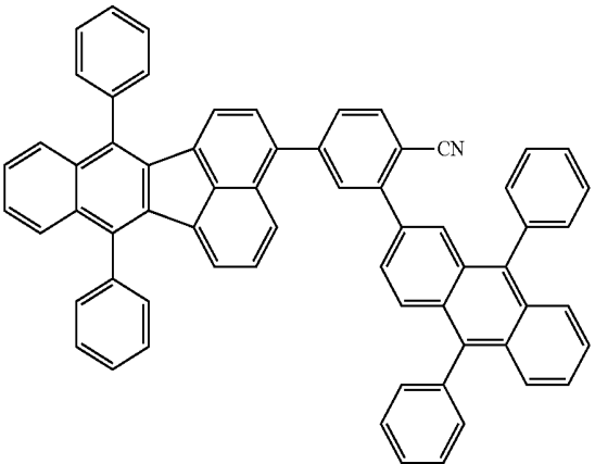
compound 25
