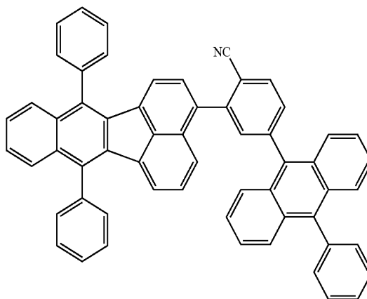
compound 19
