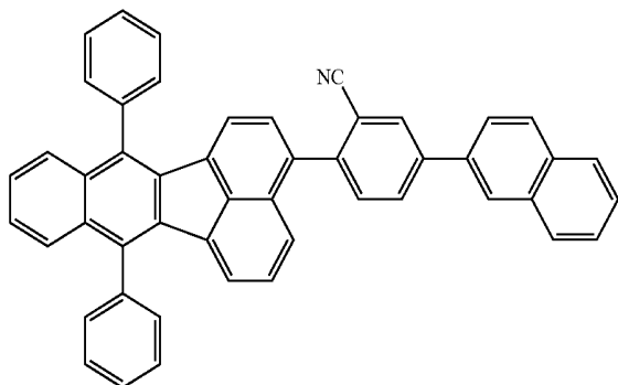
compound 13
