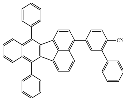
compound 22
