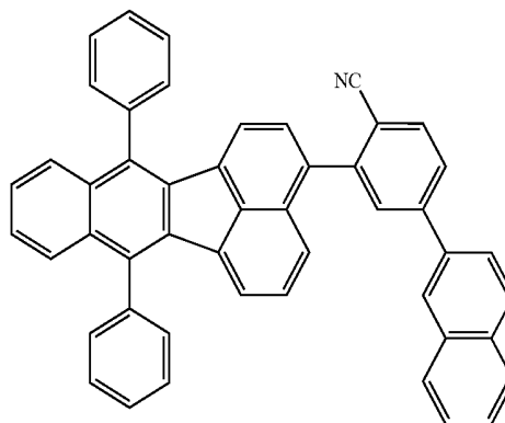
compound 18
