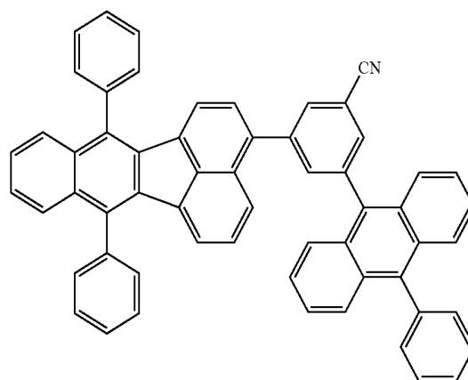
compound 10
